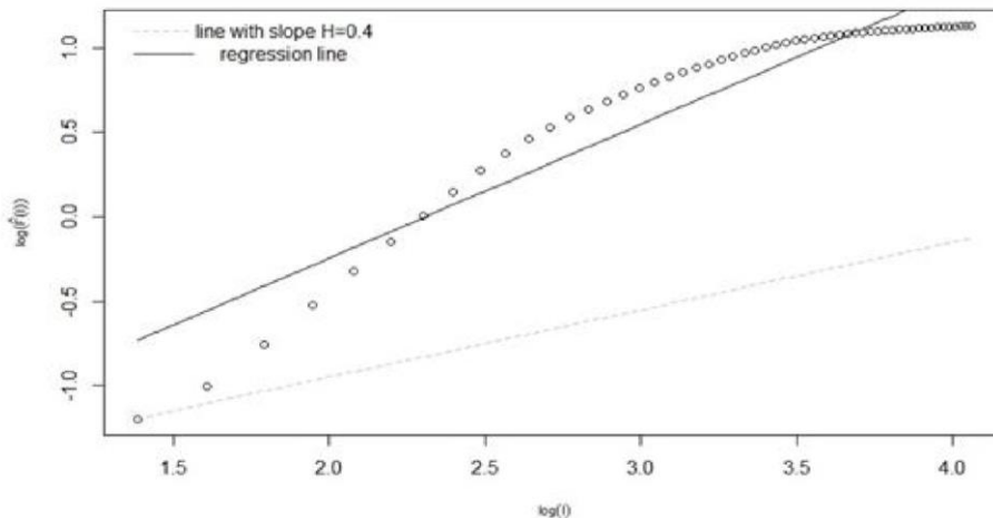
Figure 3. Plot Presenting the Scaling Properties of SDFA in -Scale for the Seismic Trace Signal of Explosion EX4.
