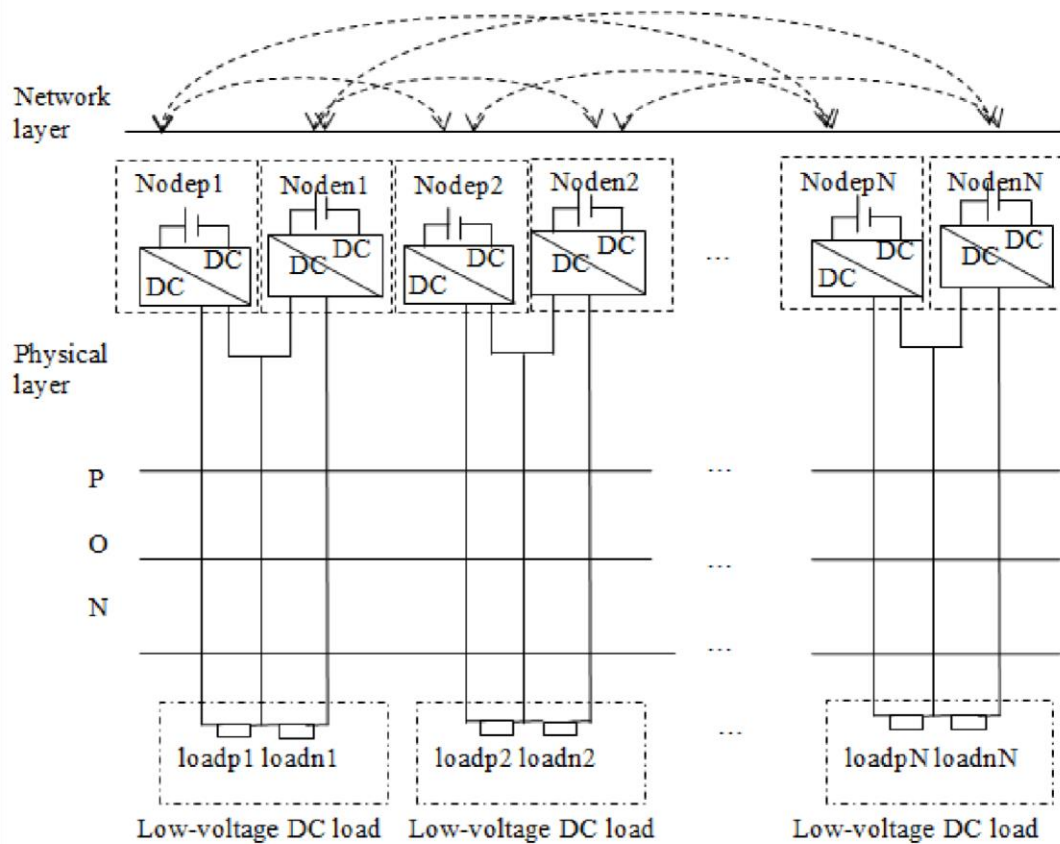
Figure 1: Schematic diagram of the power grid structure.
