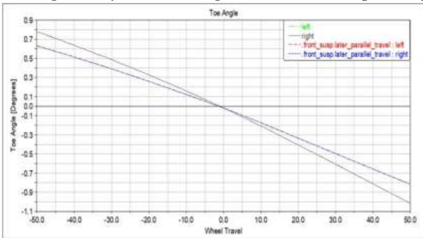
Figure.6 Simulation Curve of Parallel Double Wheel Bounce Toe Angle Change
