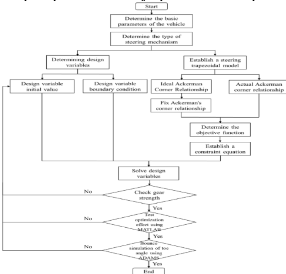
Figure. 4 Steering Trapezoid Optimization Design Flow Chart
